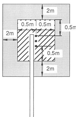
INSULATED UNSCREENED CONDUCTORS
