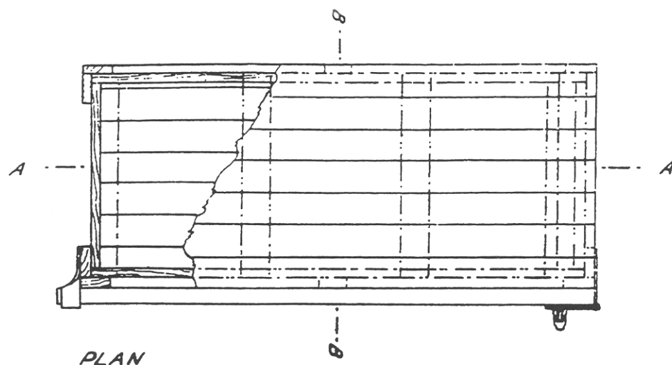
BOX FOR CONVEYANCE OF EXPLOSIVES
